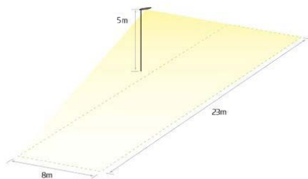
Lighting Distribution Dimensions
